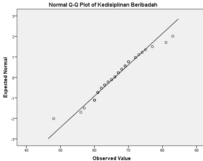
Gambar 4.1 Normal Q-Q Plot of Disiplin Ibadah
