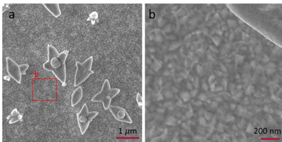
Fig. 2. ZnO nanostructure growth under the lower concentration of NaOH, i.e. 1 mL of 0.1 M. (a) low and (b) high magnification image taken at the specified area in a. Large flower-like structures are ZnO crystals that grow in the bulk solution and then drop onto the surface during the growth process.
