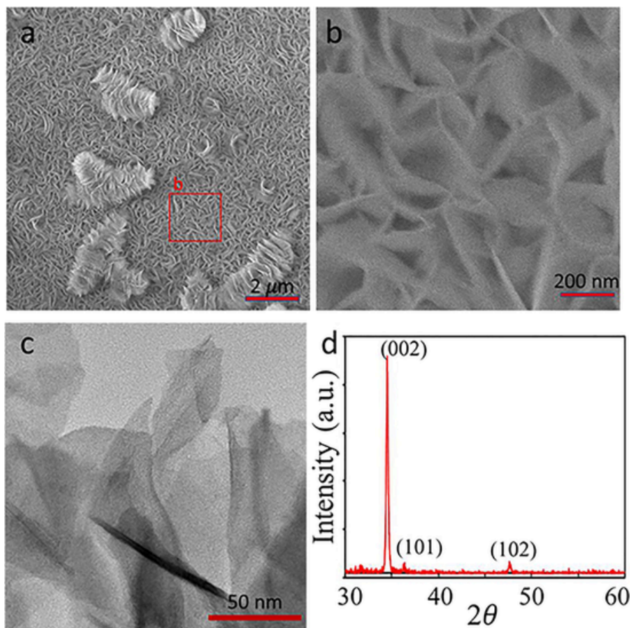
Fig. 1. (a and b) Low and high-resolution FESEM images of ZnO nanosheets on FTO substrate. (c) low-resolution TEM image. (d) X-ray diffraction pattern of the sample.
