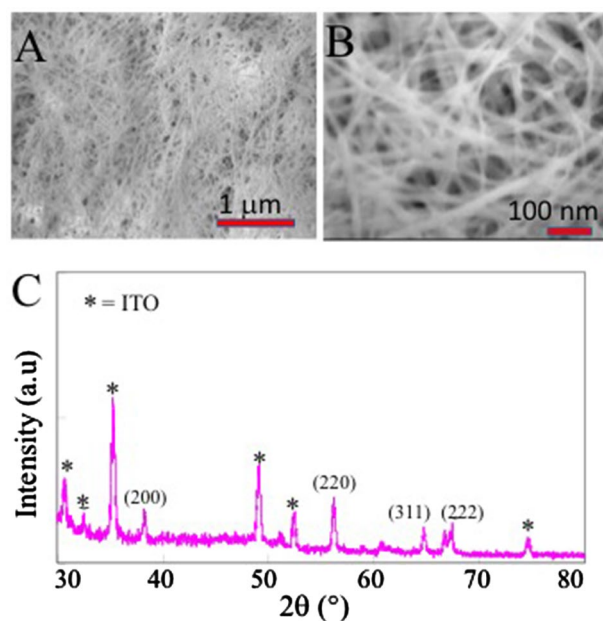
Fig. 1 (a–b) Typical FESEM image of CdO nanowires growth on the ITO surface using precursor concentration of 0.1 M. The ratio between cadmium nitrate and HMT is 1:1. (c) X-ray diffraction spectrum of CdO nanowires.
