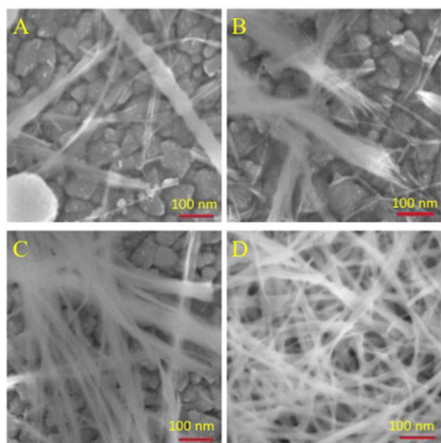
Fig. 3 Structural growth of CdO nanowires under different HMT concentrations. (a) 0.02, (b) 0.05, (c) 0.07 and (d) 0.1 M. Cadmium nitrate was fixed at 0.1 M. The growth reaction was 2 h.
