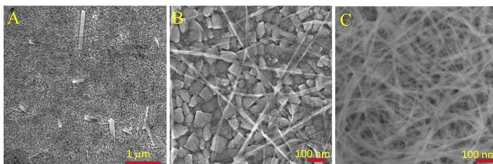
Fig. 2 Typical FESEM image of CdO nanowires grown on the ITO surface prepared using different solution concentrations, namely 0.001 (a), 0.004 (b), and 0.1 M (c). The molar ratio between the reagents in the solution was unchanged. The growth reaction time was 2 h.
